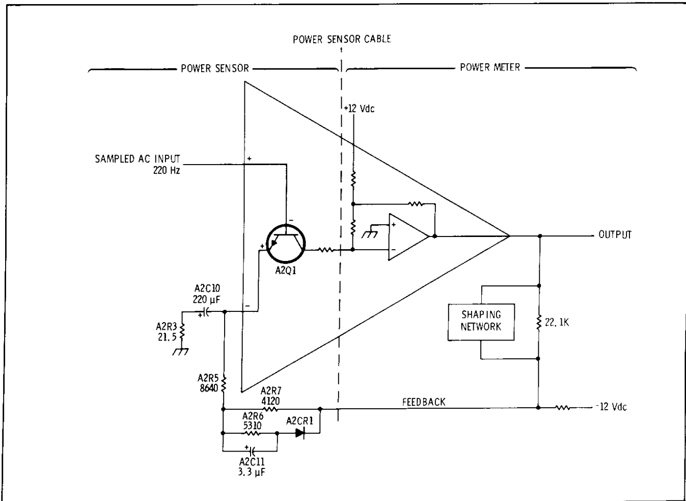
Figure 6. Operational Amplifier
